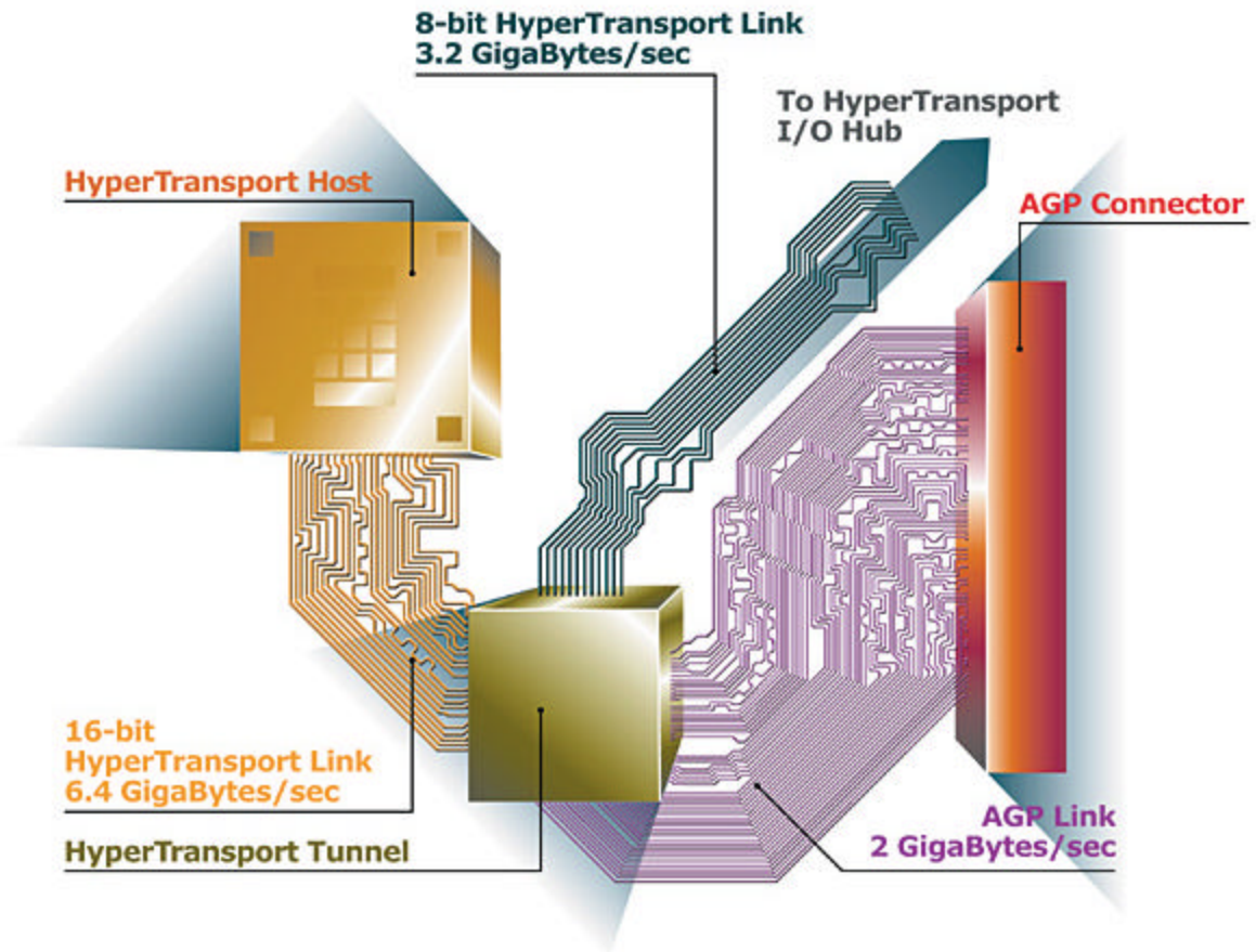
Figure 7: HyperTransport™ Technology Traces Compared to AGP Traces.
