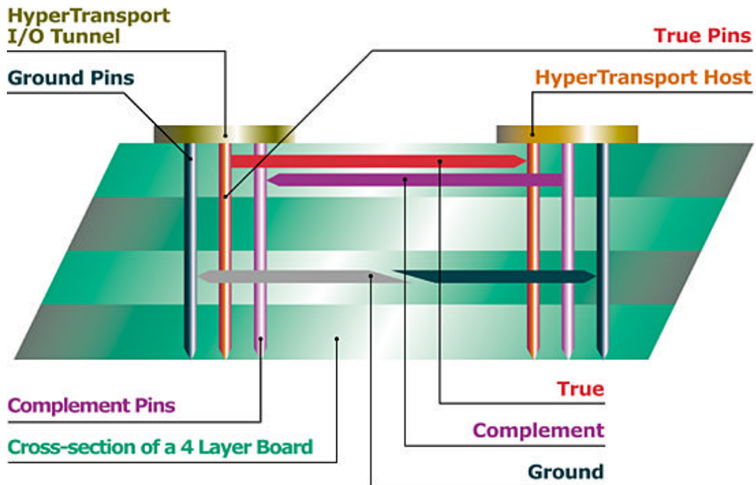
Figure 9: Return path can use compliment if ground is broken.
